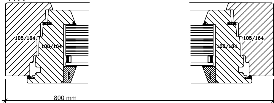
Sectional Drawing A-A
