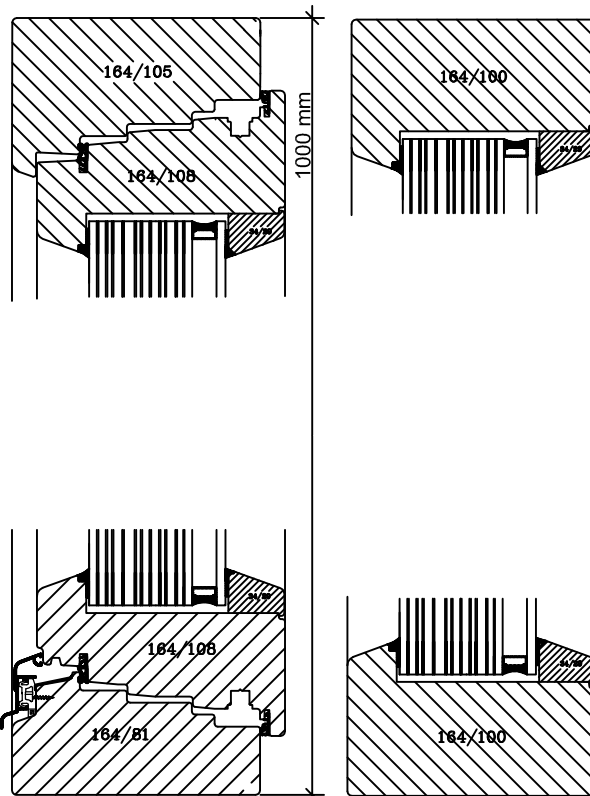
Sectional Drawing B-B
