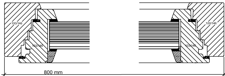
Sectional Drawing A-A
